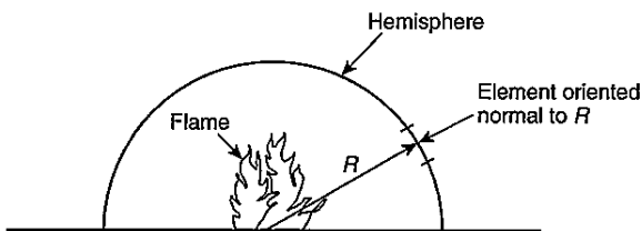
FIGURE A.5.2.5(a) Separation Distance, R .
