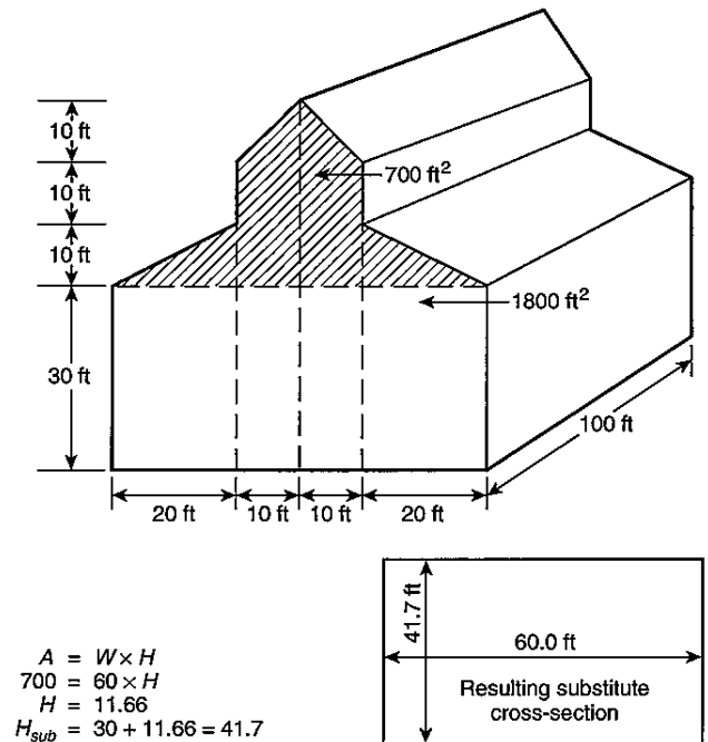
FIGURE E.3.1(a) Large Space with Nonflat Ceiling.
