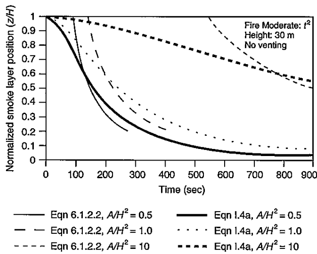
FIGURE I.4(a) Comparison of Algebraic Equations, Equations 6.1.2.2 and I.4a: t -squared Fire.
