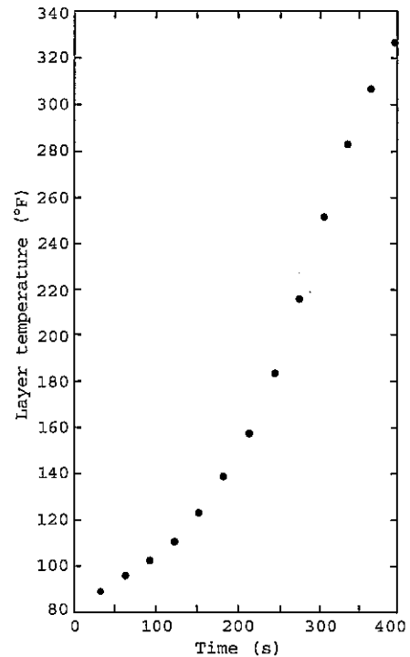
FIGURE C.7(b) Plot of the Temperature of the Smoke Layer vs. Time for the Default Simulation.
