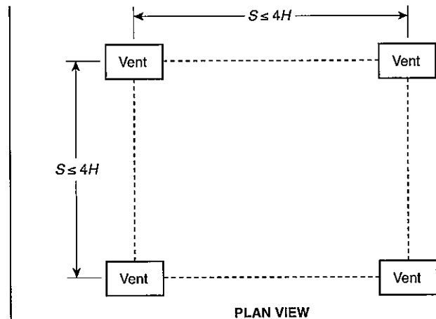
FIGURE 5.4.2(a) Vent Spacing in Rectangular Matrix (plan view).
