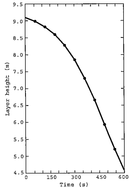
FIGURE D.10(b) Layer Height.
