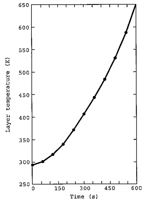
FIGURE D.10(a) Layer Temperature.
