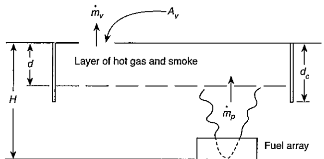
FIGURE 9.2.2.1 Schematic of Venting System.
