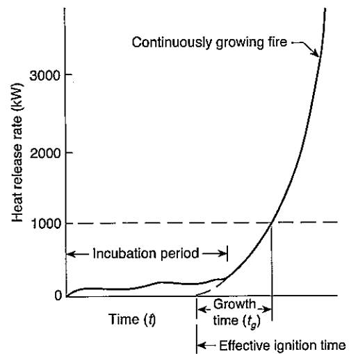
FIGURE 8.3.1 Conceptual Illustration of Continuous-Growth Fire.
